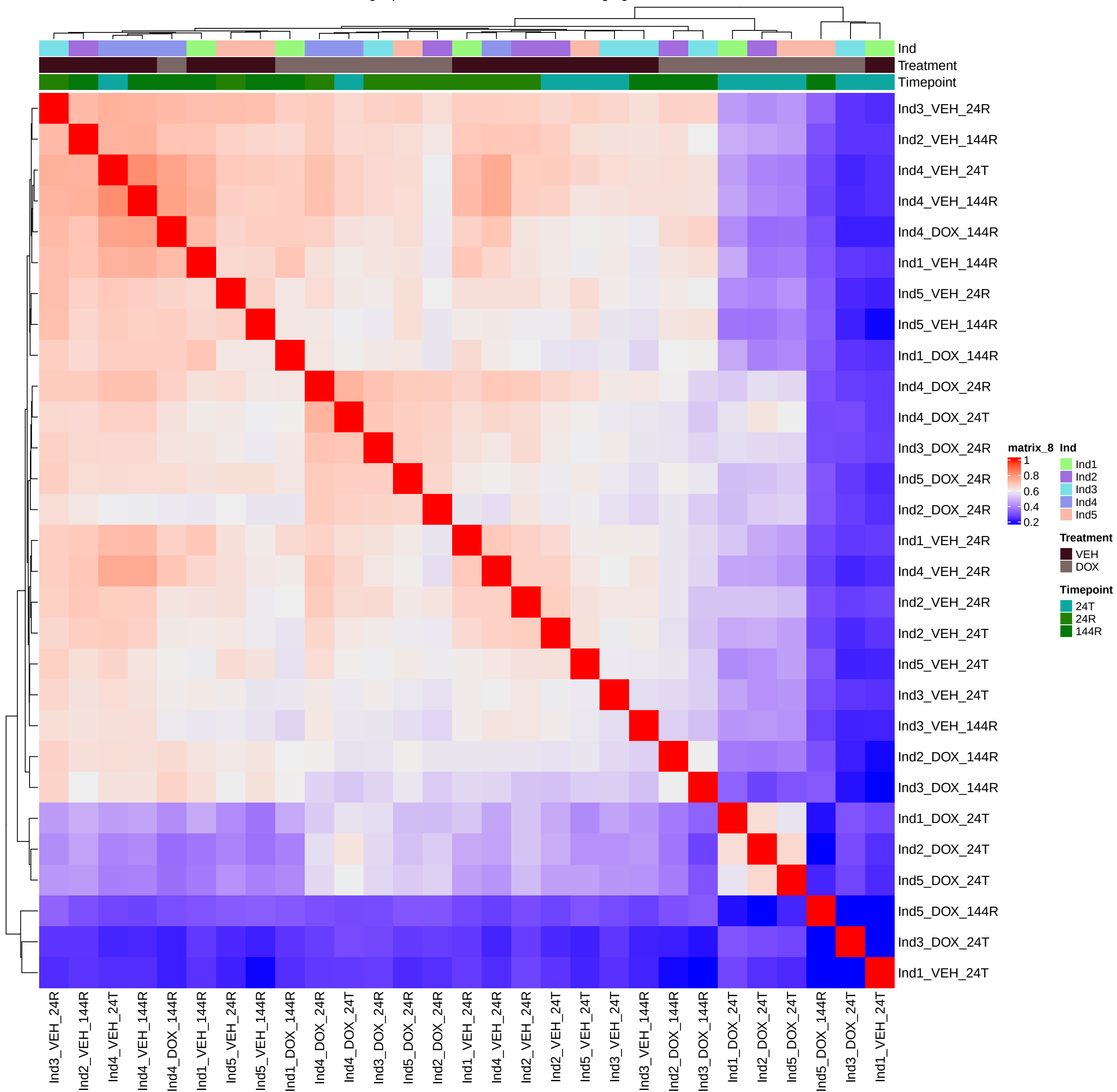
Filtered log2cpm H3K9me3 with Standard Merging
